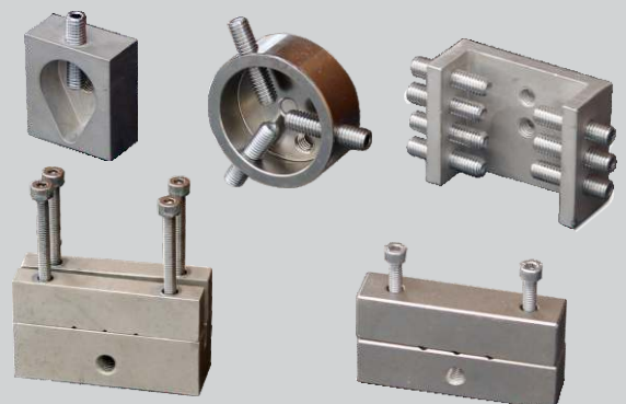
Five kinds of ( Accessories) fixtures enables the processed work piece to be sectioned at the optimal angle
