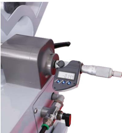
Micrometer for Cross Feed Adjustment 25 mm
